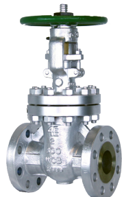
300# GATE VALVE IS 2"- 16" | BO 18"- 36" FIG.# 4E-13WCB8F
